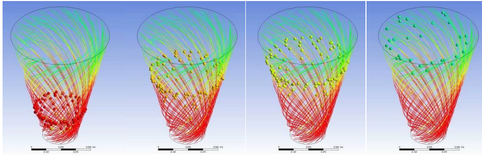
Fig. 12. Granules movement trajectories: a - W_z=1 m/s; W_r=1 m/s; W_\phi=1 m/s; b - W_z=1 m/s; W_r=1 m/s; W_\phi=15 m/s
