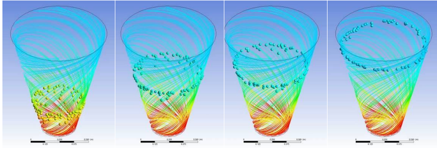
Fig. 12. Granules movement trajectories: a - W_z=1 m/s; W_r=1 m/s; W_\phi=1 m/s; b - W_z=1 m/s; W_r=1 m/s; W_\phi=15 m/s
