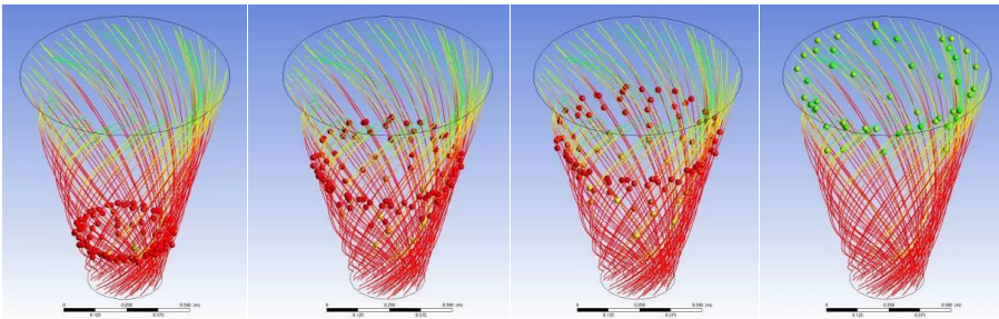
Fig. 13. Granules movement trajectories: a - W_z = 8 m/s; W_r = 1 m/s; W_\phi = 15 m/s; b - W_z = 15 m/s; W_r = 1 m/s; W_\phi = 1 m/s; c - W_z = 15 m/s; W_r = 1 m/s; W_\phi = 15 m/s
