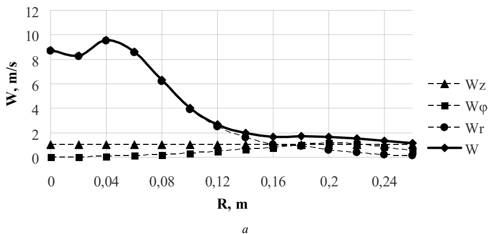
Fig. 10. Calculation of granules total speed (a) and direction of granules speed vector (b) at Q = 0,63 \text{ m}^3 / \text{s} , \varphi = 13^\circ , z = 1 \text{ m}
