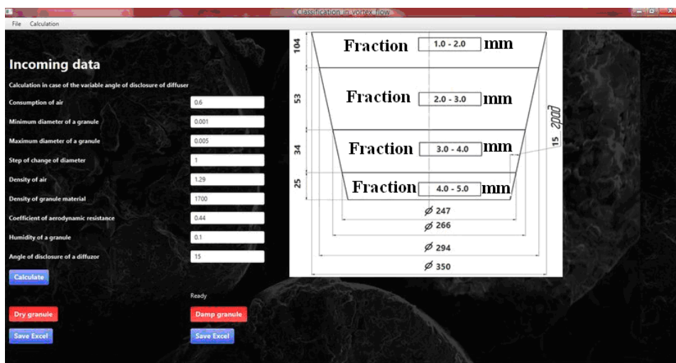
Fig. 5. The calculation of granules distribution on fractions in granulator's working space
