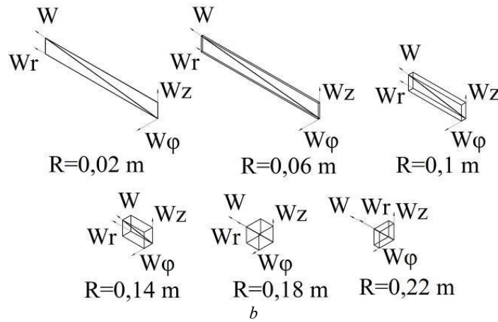
Fig. 11. Calculation of granules total speed (a) and direction of granules speed vector (b) at Q = 0,63 \text{ m}^3 / \text{s} , \varphi = 13^\circ , z = 1,2 \text{ m}
